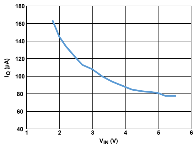
FIGURE 10. SUPPLY CURRENT (SWITCHING) ( V_{OUT} = 5\text{V} )
