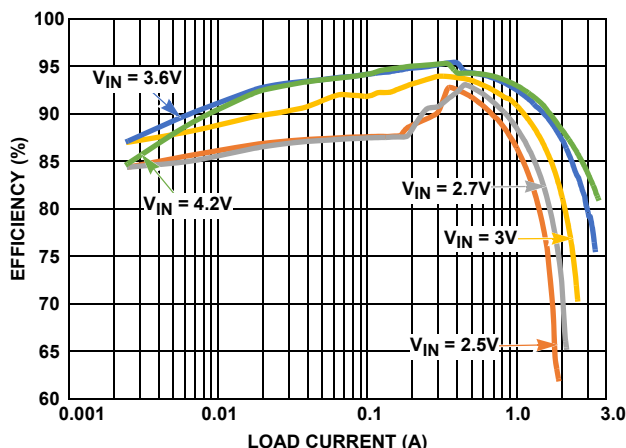
FIGURE 2. EFFICIENCY vs. OUTPUT CURRENT ( V_{OUT} = 3.3V )
