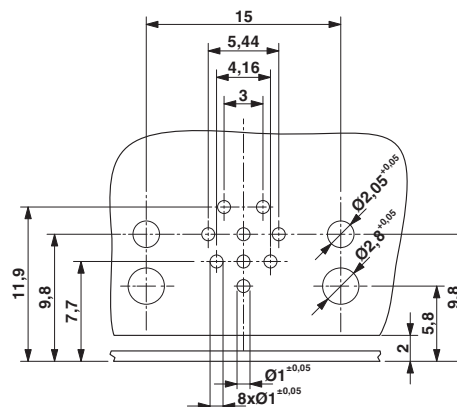
Drilling diagram only valid in connection with the SACC-M12-SCO PLUG L90 housing (order no. 1436709)
