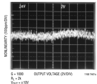
Gain Nonlinearity
