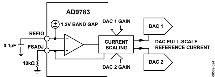
Figure 32. Reference Circuitry
