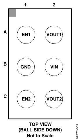
Figure 3. Pin Configuration
