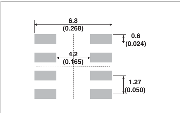
Figure 12. Footprint, dimensions in mm (inches)
