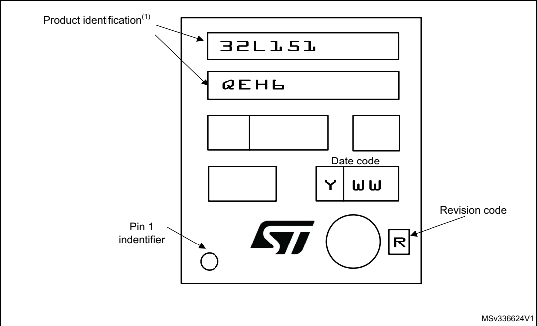
Figure 42. UFBGA132 package top view example
