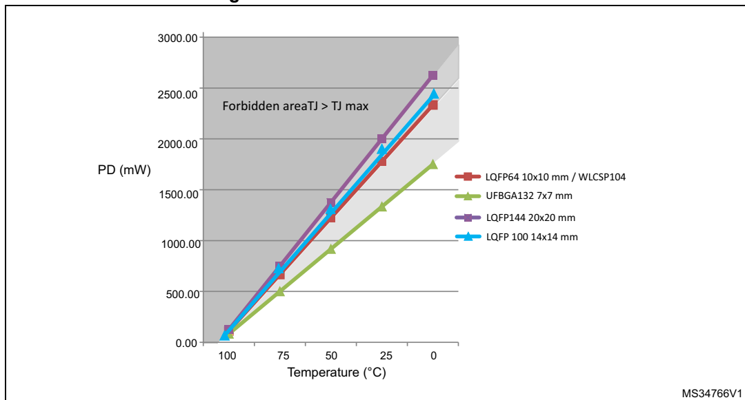
Figure 45. Thermal resistance suffix 6
