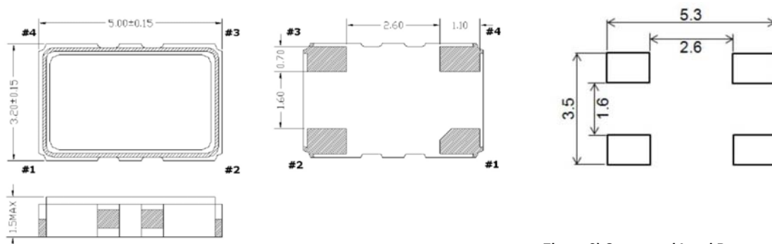
Figure 2) Suggested Land Pattern
