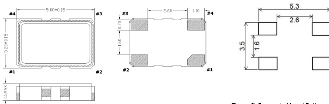
Figure 1) Top, Side and Bottom views
