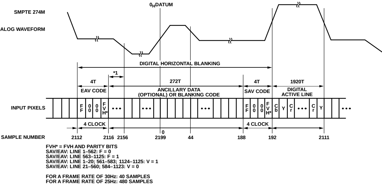
Figure 133. EAV/SAV Input Data Timing Diagram (SMPTE 274M)
