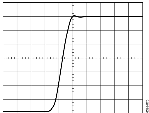
Figure 72. Output Signal from ED/HD Adaptive Filter (Mode A)
