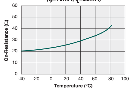
Typical On-Resistance vs. Temperature ( I_F=10\text{mA} , I_L=80\text{mA} )
