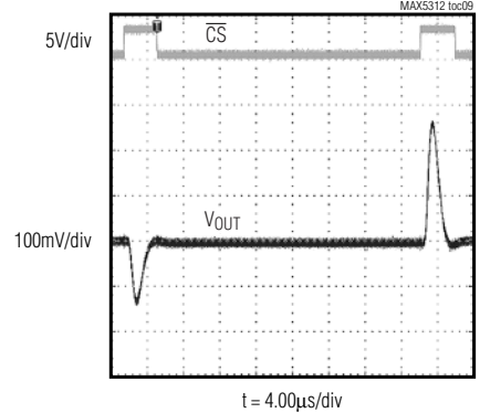
BIPOLAR MAJOR CARRY GLITCH ENERGY, CLOAD = 250pF
