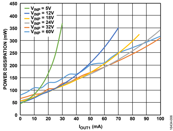
Figure 7. Power Dissipation at Various Input Voltages, T_A = +25^\circ\text{C} , V_{OUT1} = +24\text{ V} , V_{OUT2} = +5.15\text{ V} , I_{OUT2} = +7\text{ mA} , V_{OUT3} = -15\text{ V} , I_{OUT3} = -0.3\text{ mA} , T Using a Würth Elektronik 750316743 Transformer
