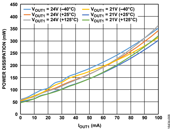
Figure 9. Power Dissipation across Temperature, V_{INP} = +24\text{ V} , V_{OUT1} = +21\text{ V} and V_{OUT1} = +24\text{ V} , V_{OUT2} = +5.15\text{ V} , I_{OUT2} = +7\text{ mA} , V_{OUT3} = -15\text{ V} , I_{OUT3} = -0.3\text{ mA} , Using a Würth Elektronik 750316743 Transformer
