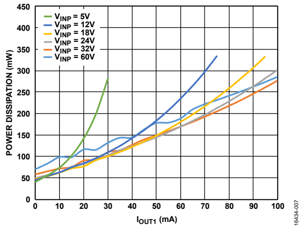
Figure 8. Power Dissipation at Various Input Voltages, T_A = +25^\circ\text{C} , V_{OUT1} = +21\text{ V} , V_{OUT2} = +5.15\text{ V} , I_{OUT2} = +7\text{ mA} , V_{OUT3} = -15\text{ V} , I_{OUT3} = -0.3\text{ mA} , Using a Würth Elektronik 750316743 Transformer
