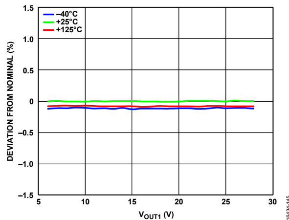
Figure 44. Inverting Regulator Line Regulation Across Temperature, V_{OUT3} = -15\text{ V} , I_{OUT3} = -7\text{ mA} , Nominal = V_{OUT3} at +24\text{ V} V_{OUT1}
