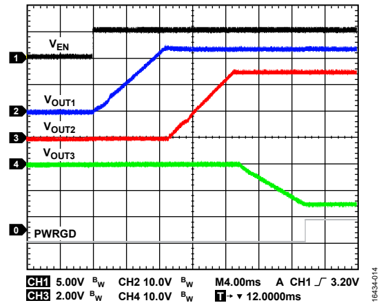
Figure 15. Power-Up Sequence at V_{EN} Rising, T_A = +25^\circ\text{C} , V_{INP} = +24\text{ V} , V_{OUT1} = +24\text{ V} , I_{OUT1} = +20\text{ mA} , V_{OUT2} = +5.15\text{ V} , I_{OUT2} = +7\text{ mA} , V_{OUT3} = -15\text{ V} , I_{OUT3} = -0.3\text{ mA}
