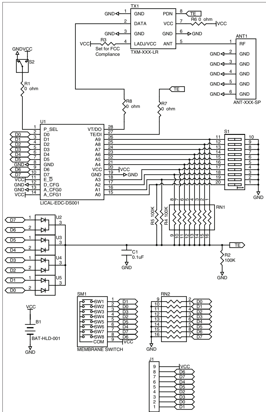
Figure 12: CMD-HHCP-***-MD Schematic
