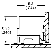
Screw type (Right-angle side)
