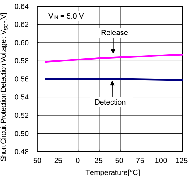
Figure 17. Short Circuit Protection Detection Voltage vs Temperature
