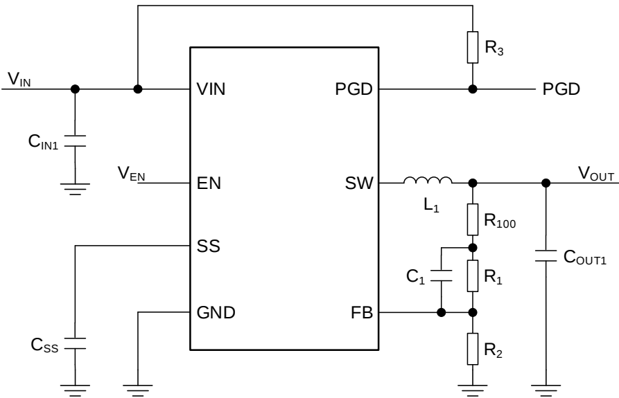
Figure 49. Reference Circuit 5
