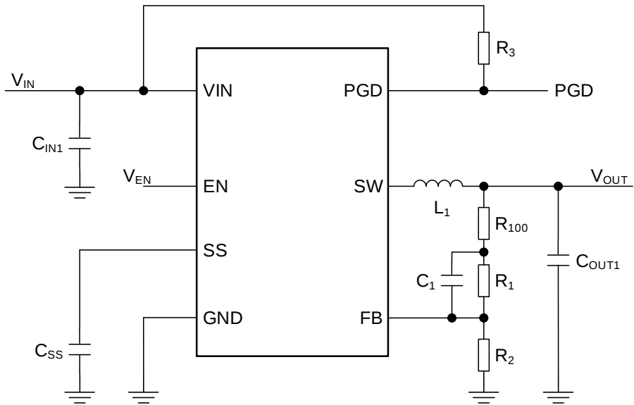
Figure 44. Reference Circuit 4
