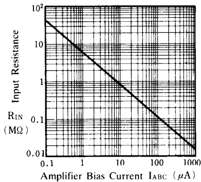
Input Resistance (Pin2.15 Open, T_a = 25^\circ\text{C} )
