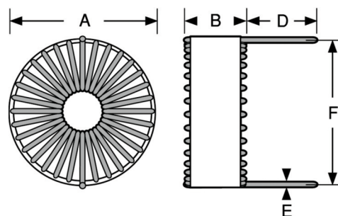
FIGURE 2: HORIZONTAL MOUNT
