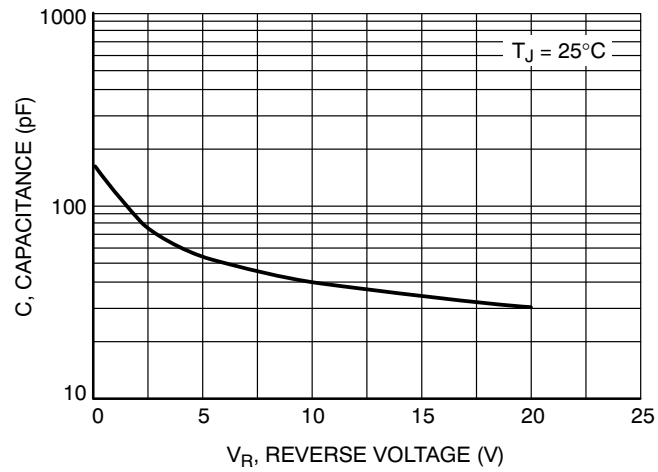
Figure 17. Capacitance
