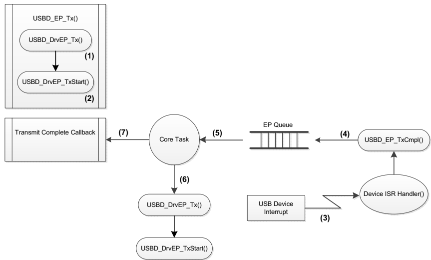
Figure 6-4 Device Asynchronous Transmit Diagram
