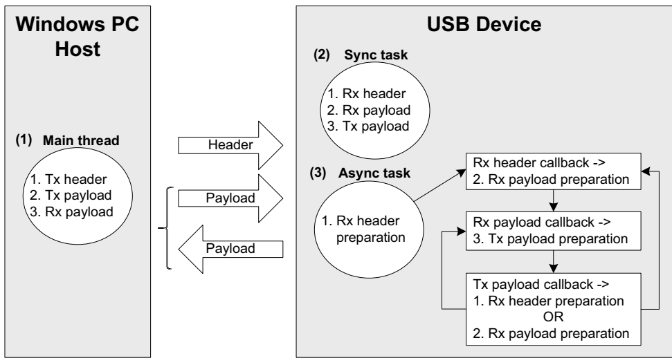
Figure 12-3 Echo Demo
