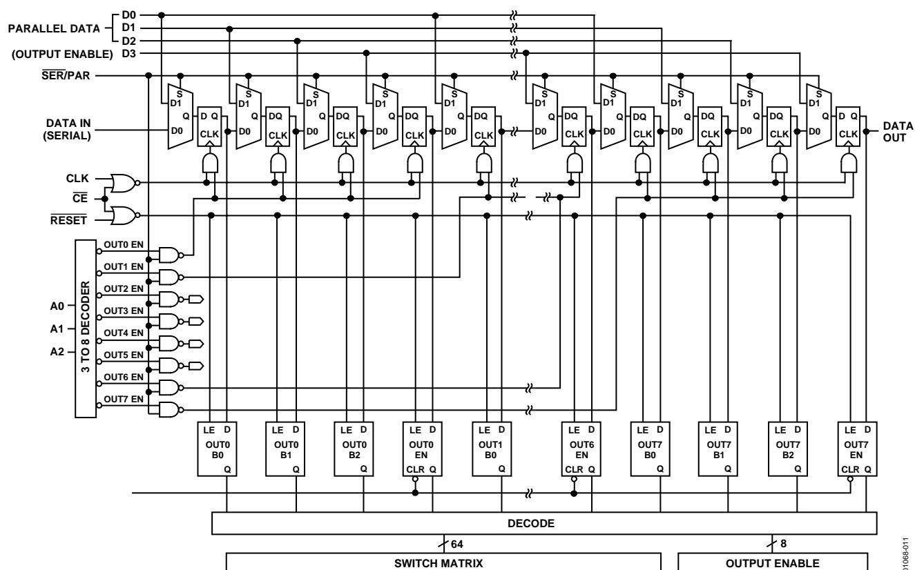
Figure 4. Logic Diagram
