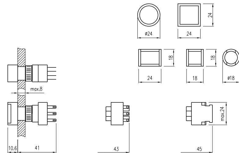
snap-action switching element with soldering-/plug-in terminal
