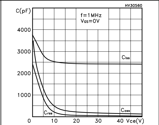
Figure 7. Capacitance variations
