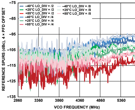
Figure 91. f_{PFD} Reference Spurs vs. VCO Frequency, 4 \times PFD Offset, Measured at LO Output, Integer Mode
