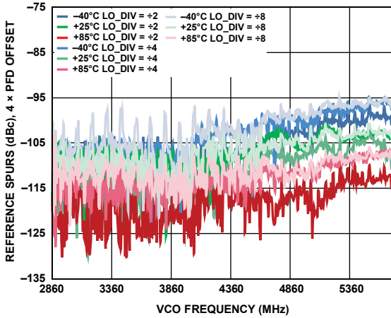
Figure 90. f_{PFD} Reference Spurs vs. VCO Frequency, 2 \times PFD Offset, Measured at LO Output, Integer Mode
