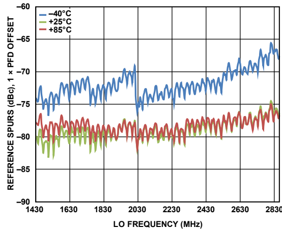
Figure 92. f_{PFD} Reference Spurs vs. LO Frequency, 1 \times PFD Offset, Measured at LO Output, Fractional Mode
