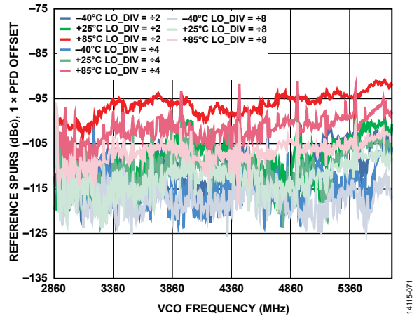
Figure 87. f_{PFD} Reference Spurs vs. VCO Frequency, 1 x PFD Offset, Measured at LO Output, Integer Mode
