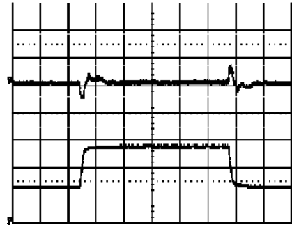
Output voltage response to load current step- change (30-60-30 A) at: T_{ref} = +25^\circ C , V_I = 5.0 V . Top trace: output voltage (100 mV/div.). Bottom trace: load current (20 A/div.). Time scale: 0.2 ms/div.
