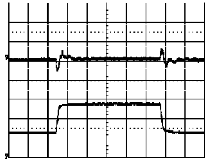
Output voltage response to load current step- change (30-60-30 A) at: T_{ref} = +25^\circ\text{C} , V_I = 5.0 V. Top trace: output voltage (100 mV/div.). Bottom trace: load current (20 A/div.). Time scale: 0.2 ms/div.
