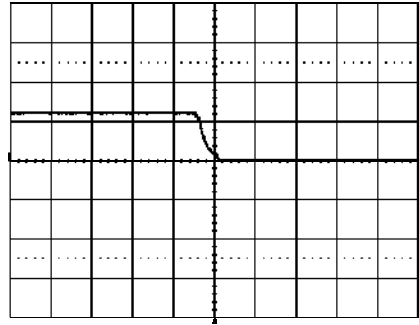
Shut-down enabled by disconnecting V_I at: T_{ref} = +25^\circ\text{C} , I_O = 60 A resistive load, V_I = 5.0 V. Top trace: output voltage (1.0 V/div.). Time scale: 0.5 ms/div.
