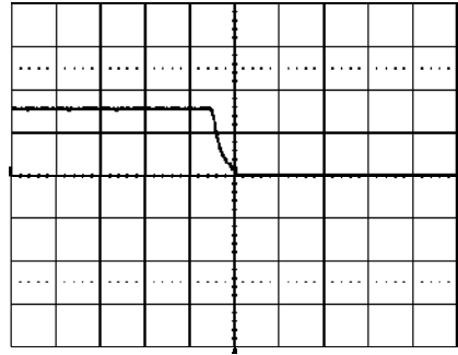
Shut-down enabled by disconnecting V_I at: T_{ref} = +25^\circ C , I_O = 60 A resistive load, V_I = 5.0 V . Top trace: output voltage (1.0 V/div.). Time scale: 0.5 ms/div.
