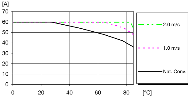
Available load current vs. ambient air temperature and airflow at V_I = 3.3 V, V_{OUT} = 2.0 V . See Thermal Consideration section.
