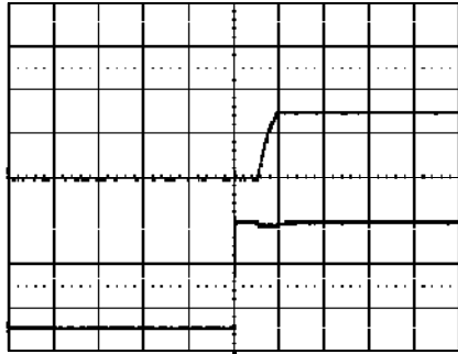
Start-up enabled by connecting V_I at: T_{ref} = +25^\circ C , I_O = 60 A resistive load, V_I = 5.0 V . Top trace: output voltage (1.0 V/div.). Bottom trace: input voltage (2.0 V/div.). Time scale: 10 ms/div.
