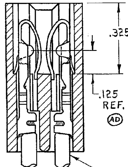
SECT. A-A SCALE 4-1 CONTACT REF. ONLY
