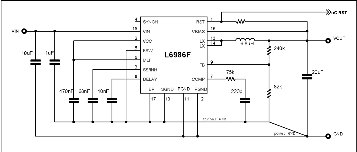
Figure 1. Application schematic
