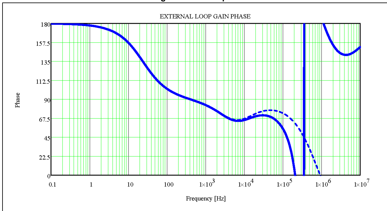
Figure 33. Phase plot
