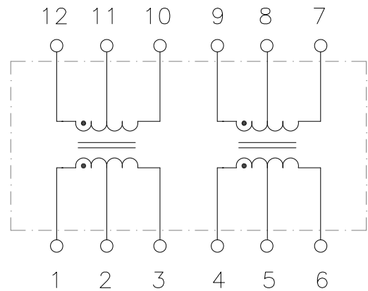
Circuit B
