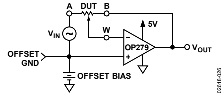
Figure 26. Inverting Gain
