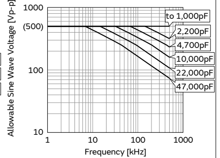
Chip (L×W): 3.2×1.6mm, 3.2×2.5mm 4.5×3.2mm, 5.7×5.0mm U2J (7U) char., Rated Voltage: DC500V
