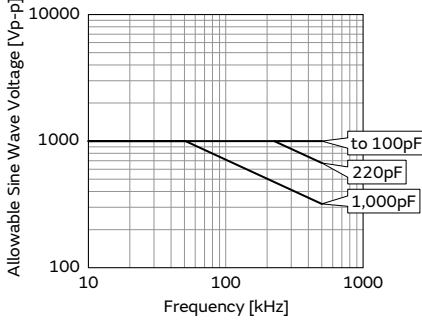
Chip (L×W): 3.2×1.6mm COG char., Rated Voltage: DC1kV
