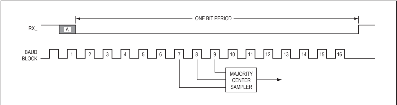
Figure 6. Midbit Sampling
