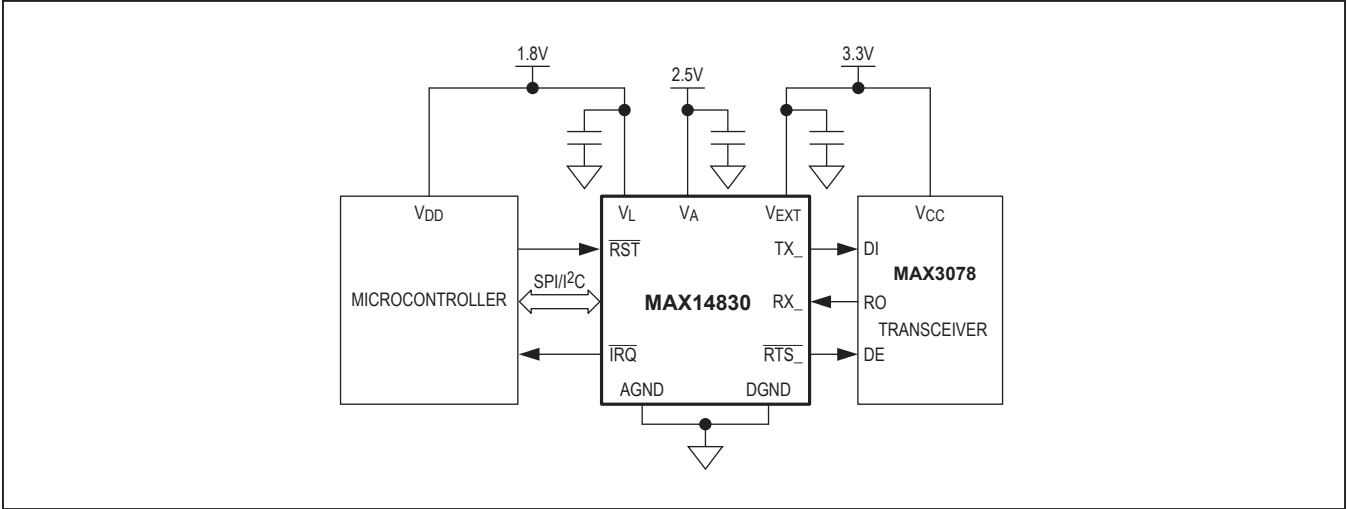
Figure 28. Logic-Level Translation
