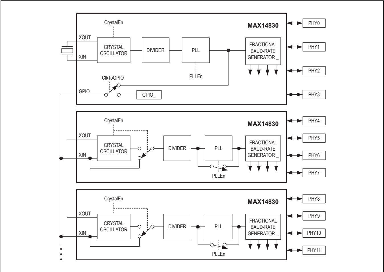
Figure 29. Interchip Synchronization
