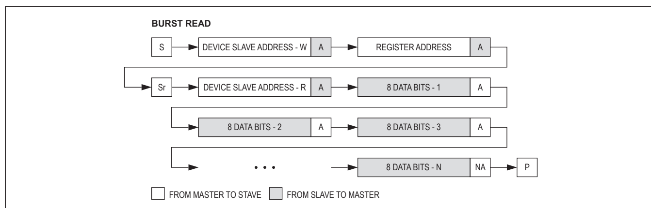
Figure 25. Burst Read Sequence
