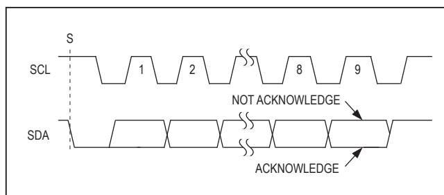
Figure 26. Acknowledge Bits
