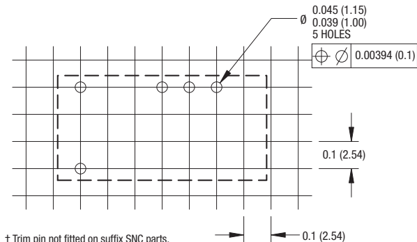
14 Pin DIP Package
