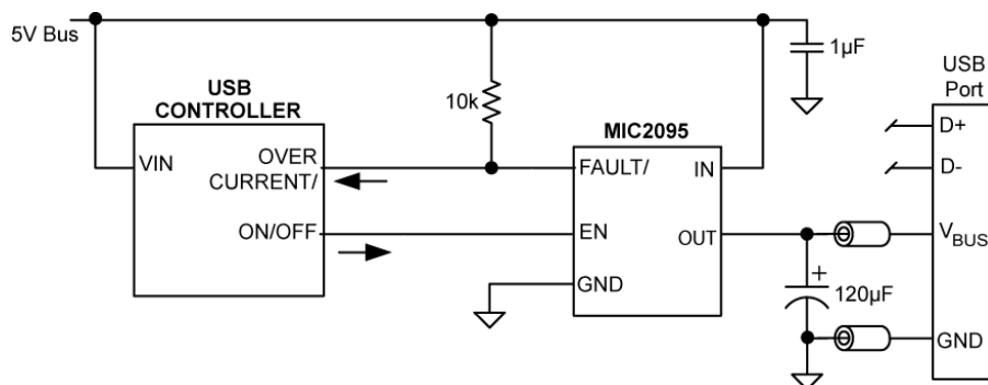
MIC2095 USB Power Switch
