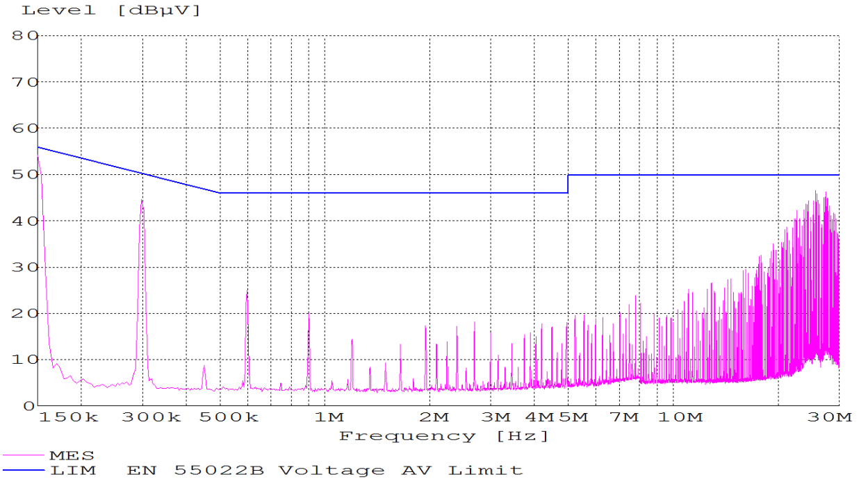
Figure 23. EMC Considerations
