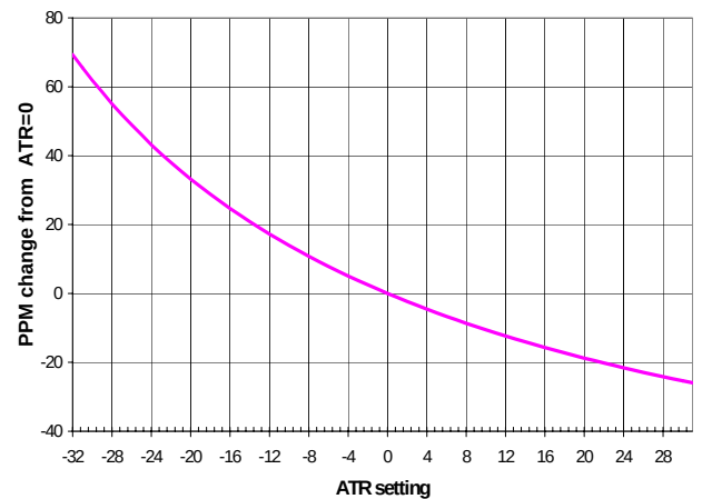
FIGURE 10. \Delta F_{OUT} vs ATR SETTING
