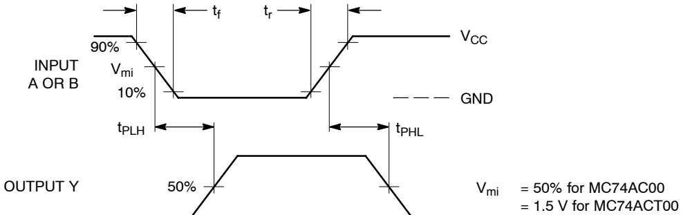
Figure 3. Switching Waveforms
