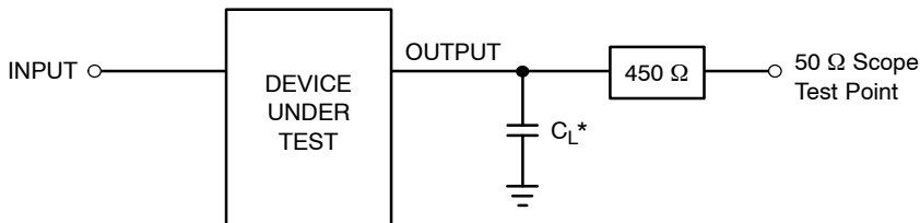
Figure 4. Test Circuit
