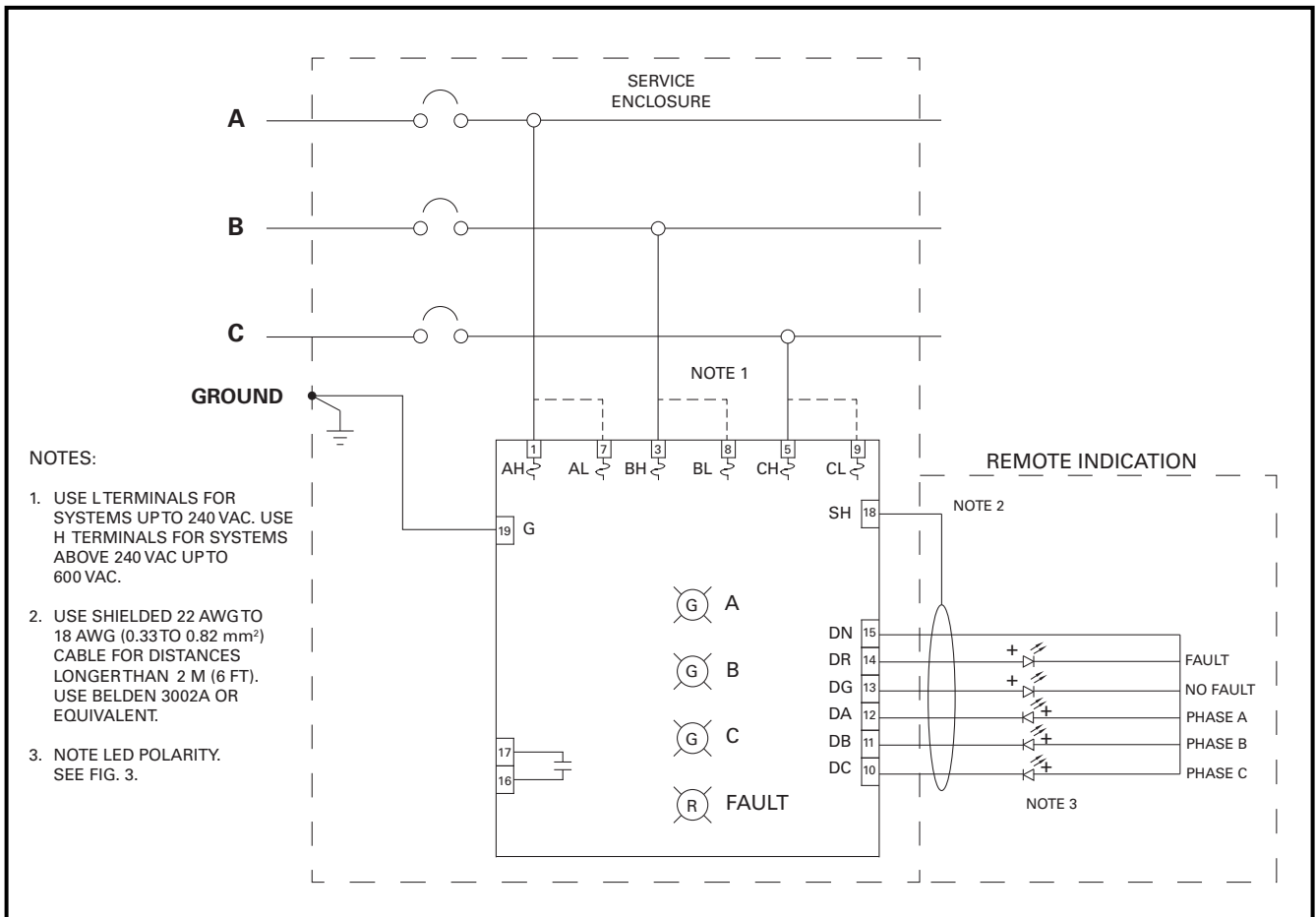
FIGURE 2. Connection Diagram.
