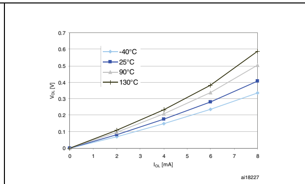
Figure 26. Typ. V_{OL} @ V_{DD} = 1.8 V (high sink ports)
