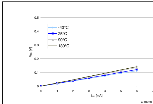
Figure 27. Typ. V_{OL} @ V_{DD} = 3.0 V (true open drain ports)
