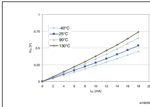
Figure 25. Typ. V_{OL} @ V_{DD} = 3.0 V (high sink ports)
