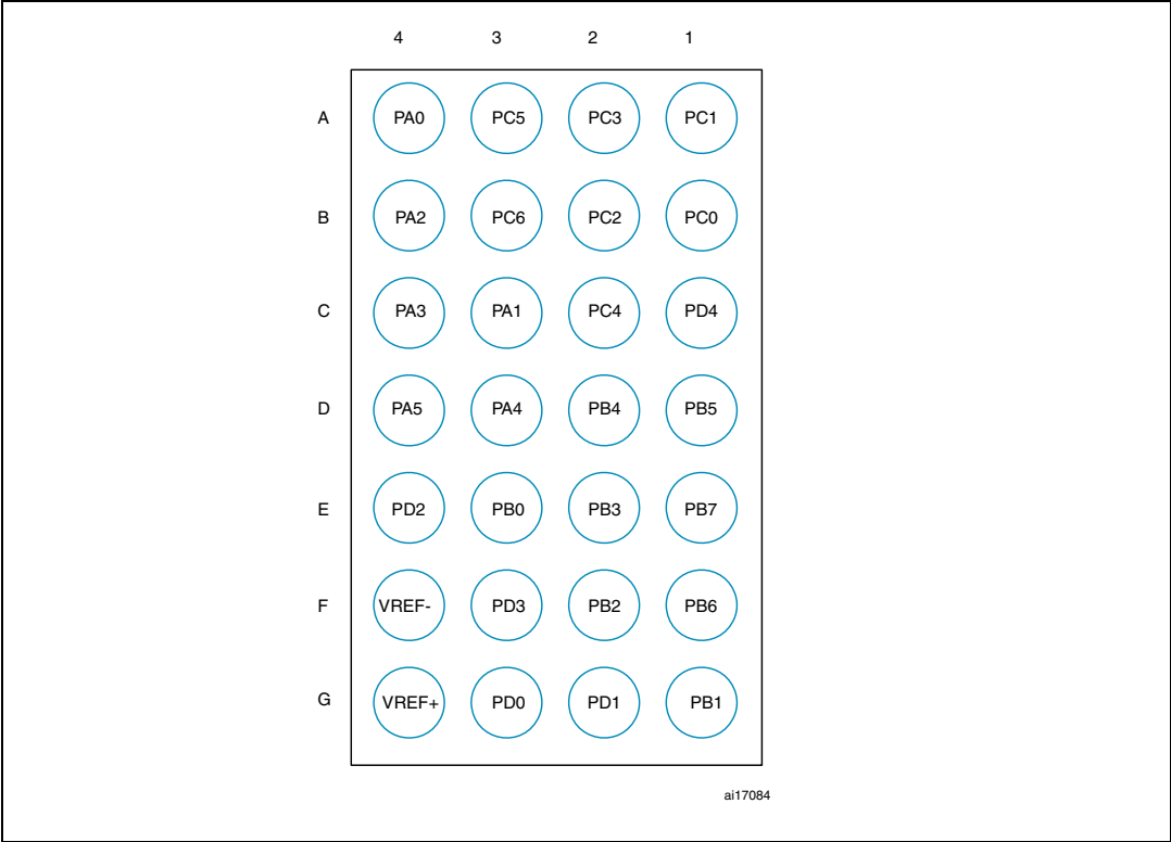
Figure 6. STM8L151Gx WLCSP28 package pinout
