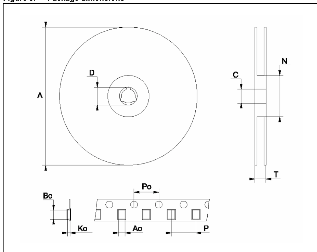
Figure 3. Package dimensions
