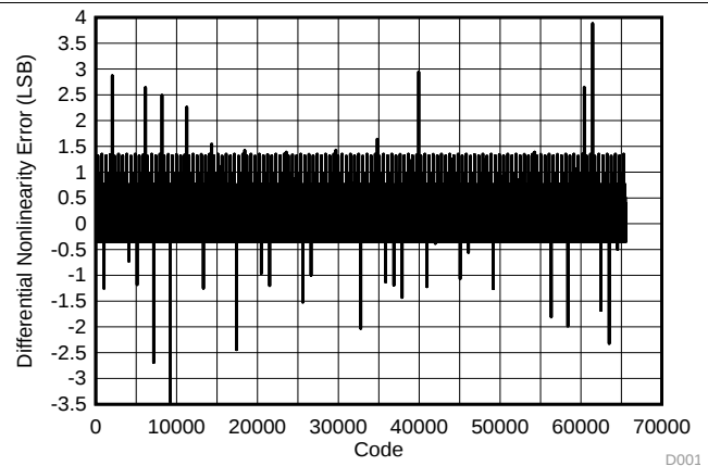
Figure 2. Differential Nonlinearity
