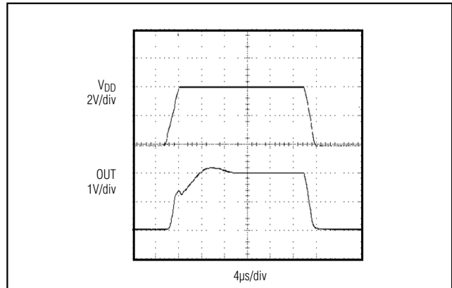
Figure 5. Power-Up/Down Waveform
