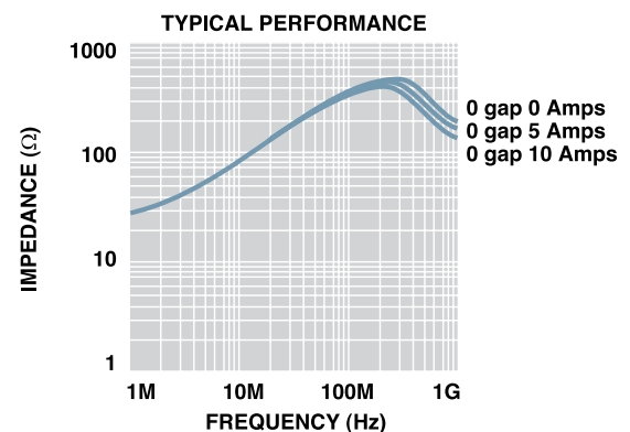
Gap effect of ferrite subjected to direct current.
