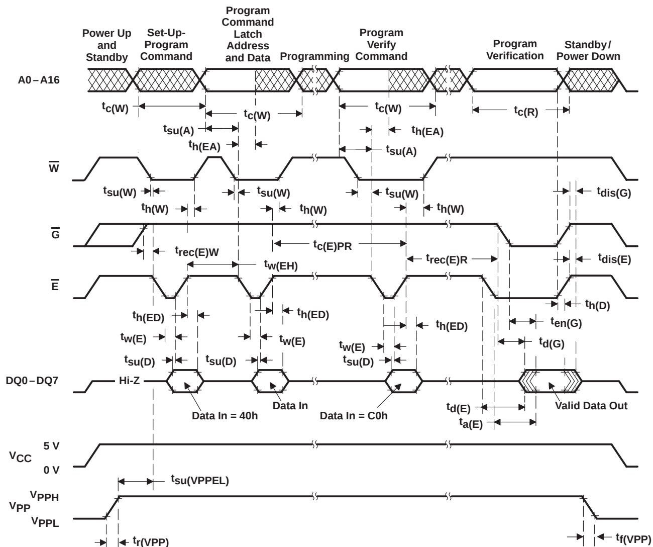
Figure 9. Write-Cycle (Alternative \bar{E} -Controlled Writes) Timing
