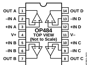
Figure 3. 14-Lead PDIP (P-Suffix) 14-Lead Narrow-Body SOIC (S-Suffix)
