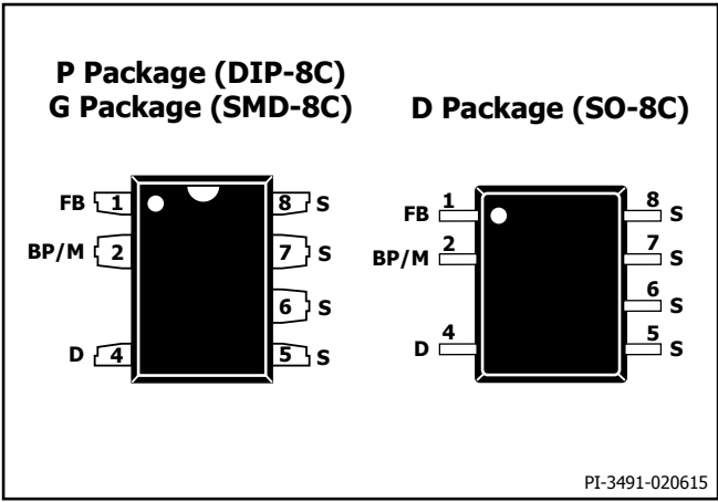
Figure 4. Pin Configuration.
