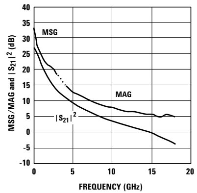
Figure 17. MSG/MAG and |S_{21}|^2 vs. Frequency at 3V, 60 mA.
