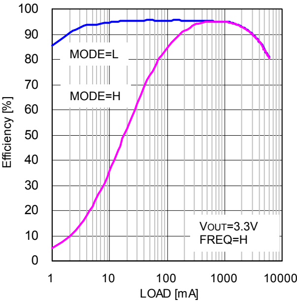
Figure 9. Efficiency vs Load Current (VIN=5V, VOUT=3.3V, L=1.0μH, FREQ=H)
