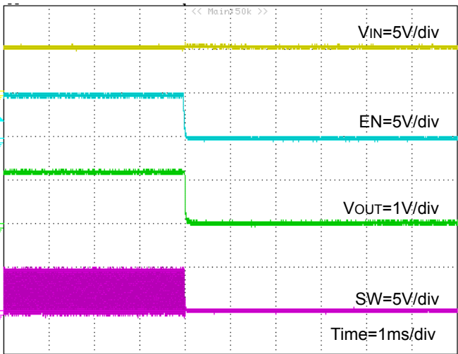
Figure 29. Power Down Waveform with EN (FREQ=H, RLOAD=0.2Ω)
