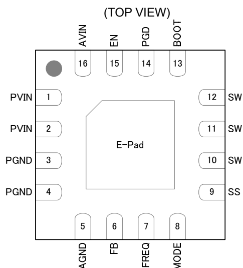
Figure 2. Pin Assignment
