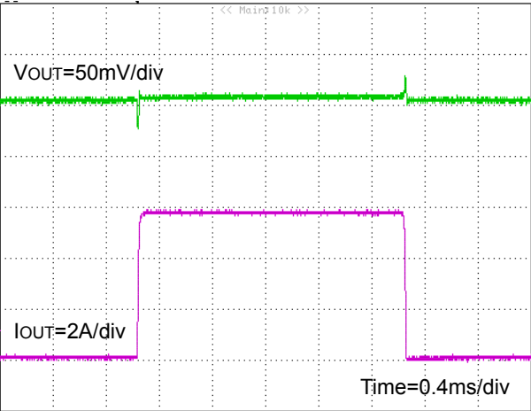
Figure 39. Load Transient Response IOUT=0.1A to 6A (VIN=5V, VOUT=1.2V, FREQ=L, MODE=H, COUT=Ceramic 44μF)
