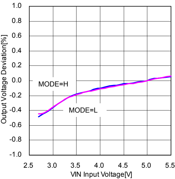
Figure 36. Line Regulation (VOUT=1.2V, L=1.0μH, FREQ=H, IOUT=6A)
