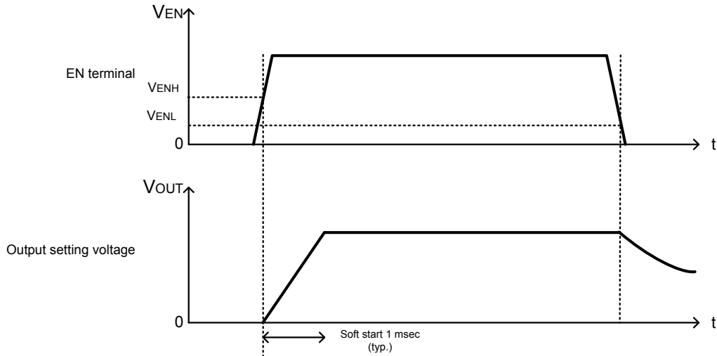
Figure 43. Start Up and Down with Enable
