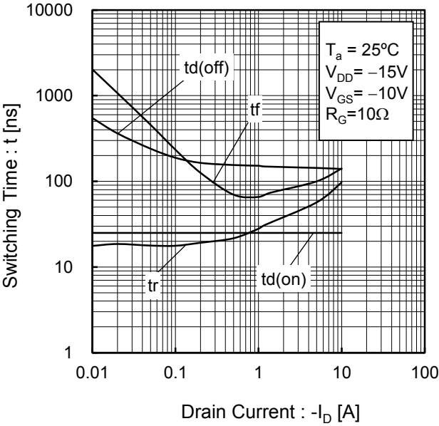
Fig.21 Switching Characteristics
